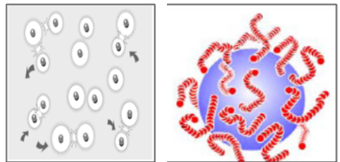
Figure 1. a) Electrostatic push b) Steric push
