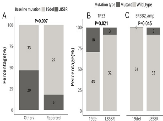
Figure 4. EGFR 19del-mutant patients acquired significantly more mutations in the MAPK/PI3K pathway ( P=0.007 ) and TP53 ( P=0.021 ), while ERBB2 amplifications were only detected from L858-mutant patients ( P=0.045 ). Histograms illustrating the acquired mutations detected among 19del and L858R-mutant patients in A. MAPK/PI3K pathway; B. TP53 and C. ERBB2 amplification. Reported includes only specific mutations already established in the development of osimertinib or EGFR -TKI resistance, Others refers to mutations that have not been associated with the EGFR -TKI resistance mechanism.
