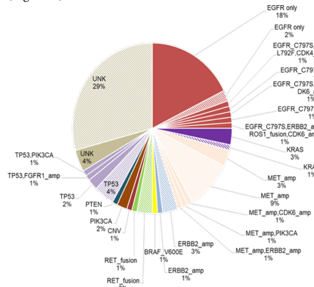
Figure 2. Distribution of the osimertinib-treated patients according to the major acquired mutations. Shaded slices refer to those with T790M loss.
